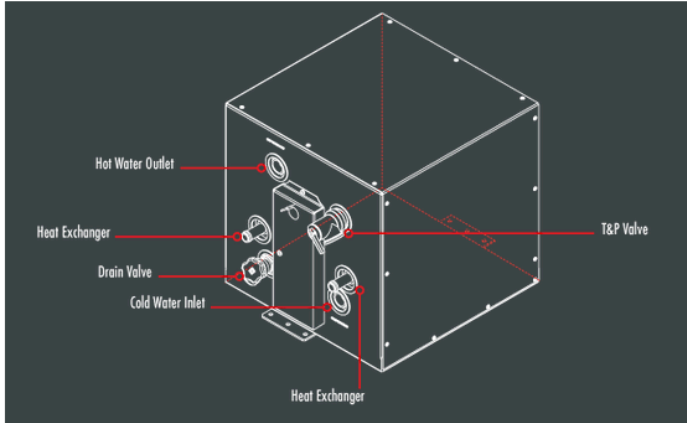
11 GAL Side Mount, 120V, Front Heat Exchange 11840
