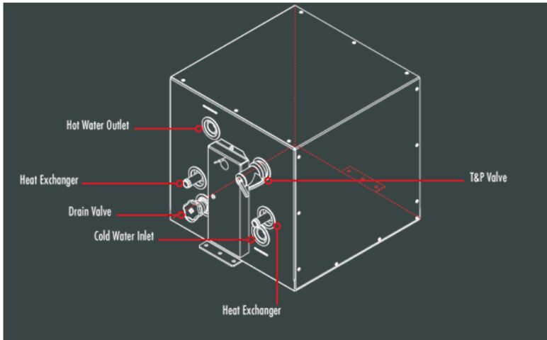
6 GAL Side Mount, 120V, Front Heat Exchange 11810
